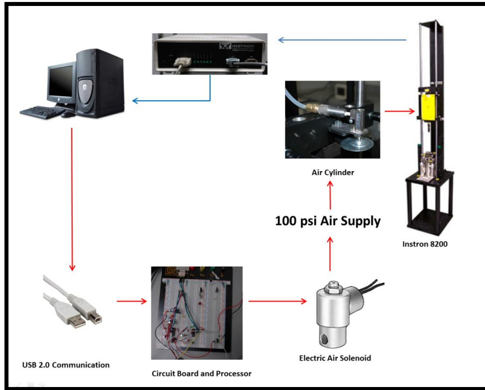
Figure 2.24: Time-Coordinated Impact Test Set-Up
