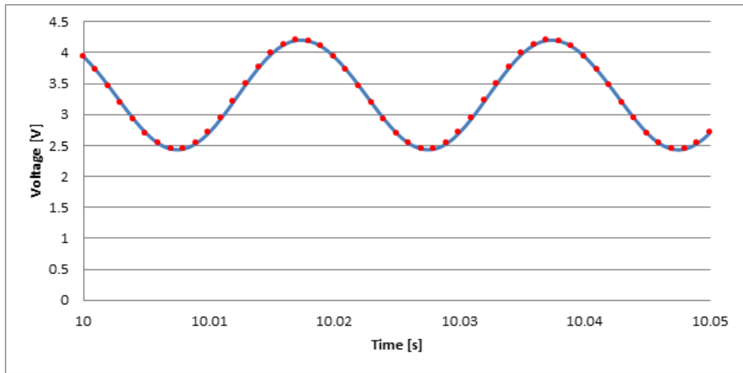
Figure 3.31: Symmetric Cross-Ply Sample #17: Voltage vs. Time, \omega = 50 Hz, I_{\text{avg}} = 75 A
