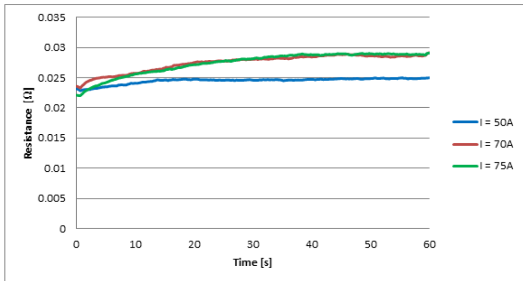
Figure 3.10: Unidirectional Sample #14: Resistance vs. Time, Steady Current
