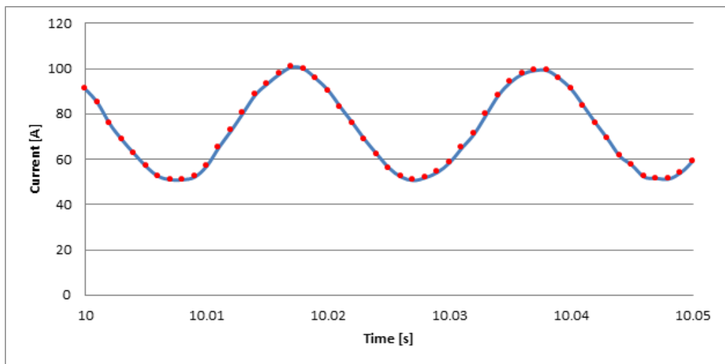
Figure 3.32: Symmetric Cross-Ply Sample #17: Current vs. Time, \omega = 50 Hz, I_{\text{avg}} = 75 A
