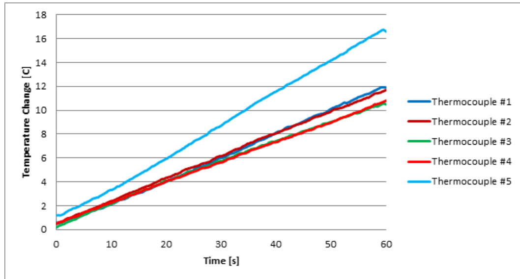
Figure 3.50: Symmetric Cross-Ply Sample #17: Temperature Change vs. Time, Steady Current: I = 50 A
